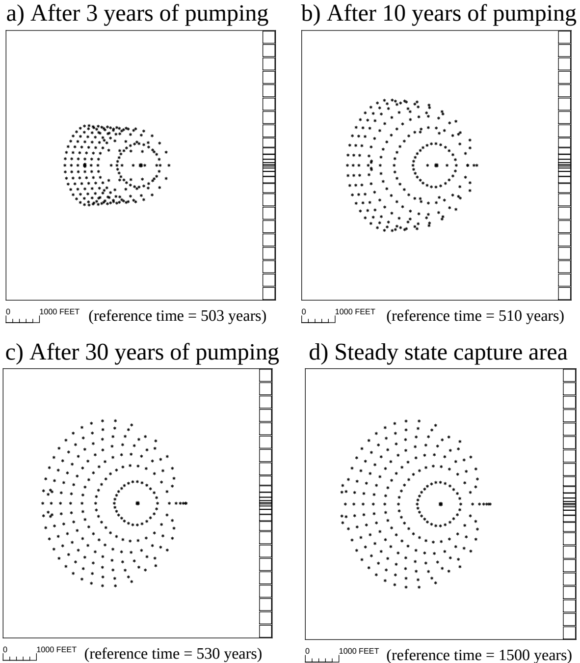
Figure 6-13. Evolution in time of the capture area for the well located in layer 1.
