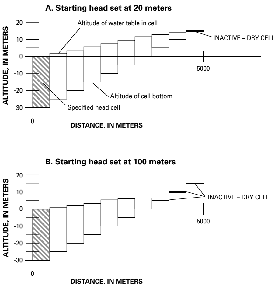
Figure 5. Cross-sectional view of a finite-difference representation simulating a variable thickness ground-water system with flow to a specified head due to areal recharge: (A) starting head set at 20 meters, and (B) starting head set at 100 meters.
