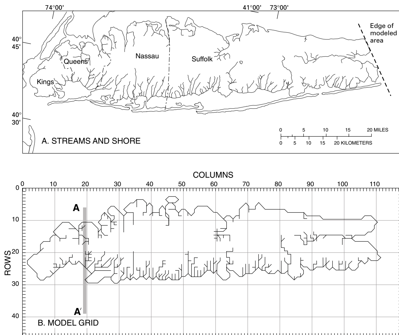
Figure 18. Areal representation of Long Island, New York, by the regional ground-water flow model: (A) Actual map view; and (B) Discretized map view. (Modified from Buxton and Smolensky, 1999)
