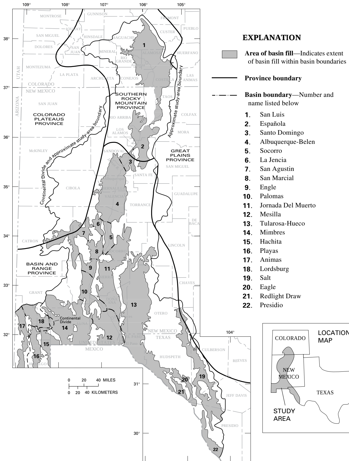
Figure 7. Location of the alluvial basins studied by the Southwestern Alluvial Basins Regional Aquifer-Systems Analysis. The basins along the Rio Grande form a continuous stretch of alluvial deposits. (Modified from Wilkins, 1998)
