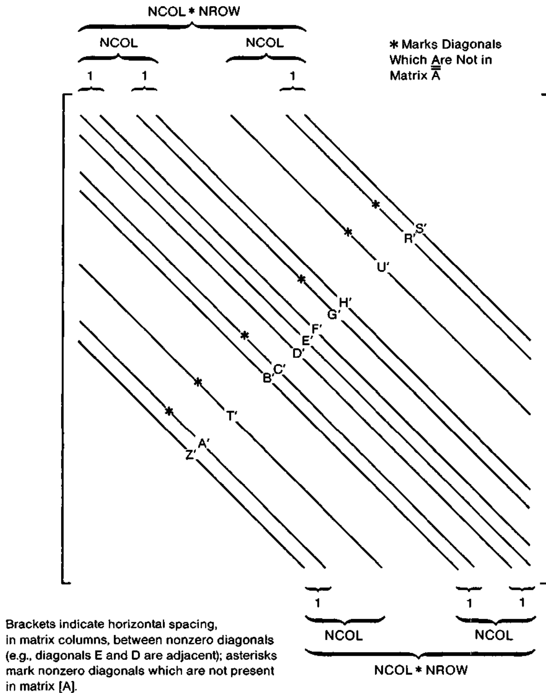
Figure 50.—Structure of matrix [A+B] showing nonzero diagonals.
